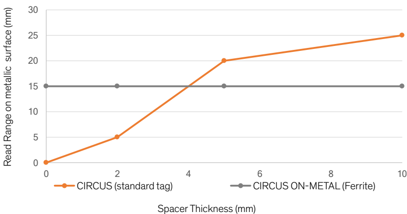
Comparison standard inlays with spacer and inlays with ferrite material
